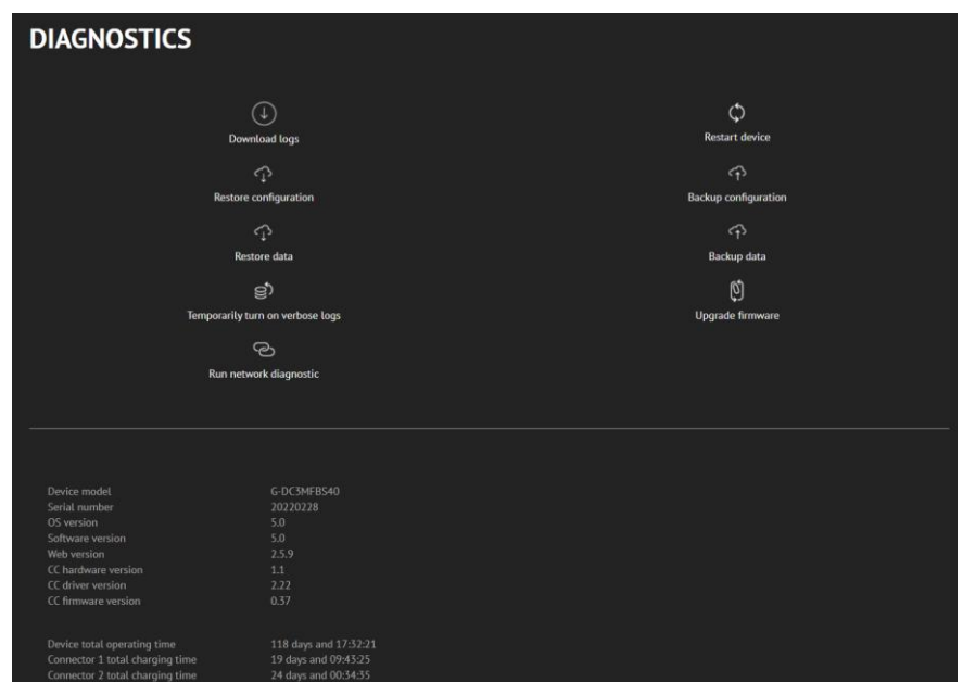
Figure 38: Diagnostics web interface module
