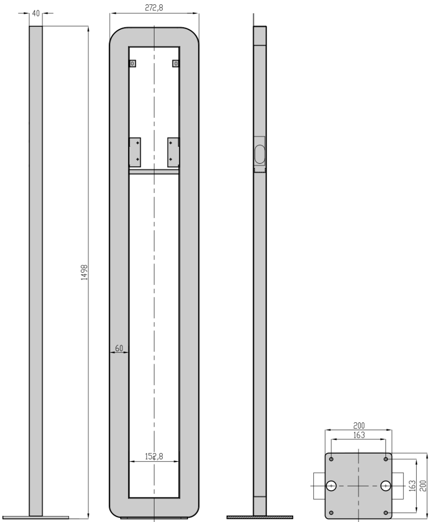
Figure 7: INCH mounting pole
