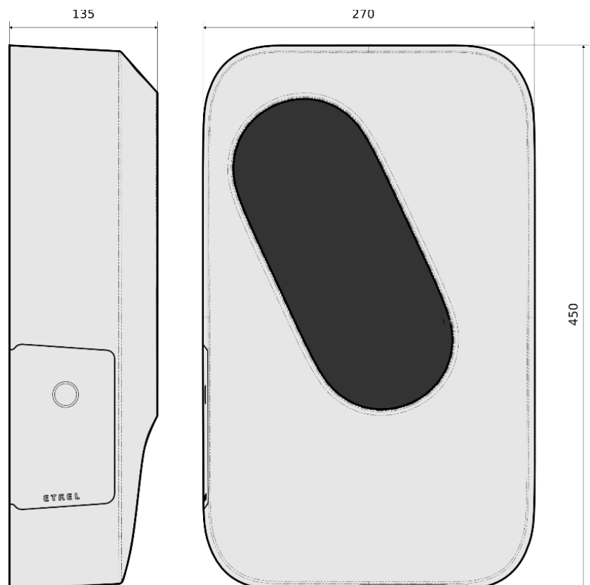
Figure 5: Dimensions of INCH charging station
