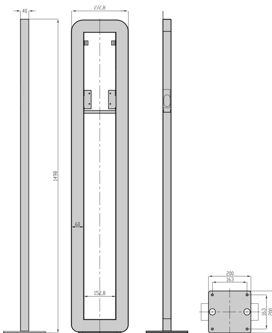
Figur 6: INCH monteringsstang
